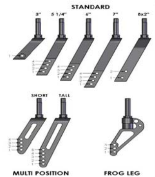
FIGURE 3: CASTER OPTIONS
