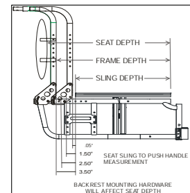
FIGURE 1: DEPTH ADJUSTABLE BACK FRAME
