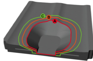
Optiwell shape and variable PLA (Pelvic Loading Area)
